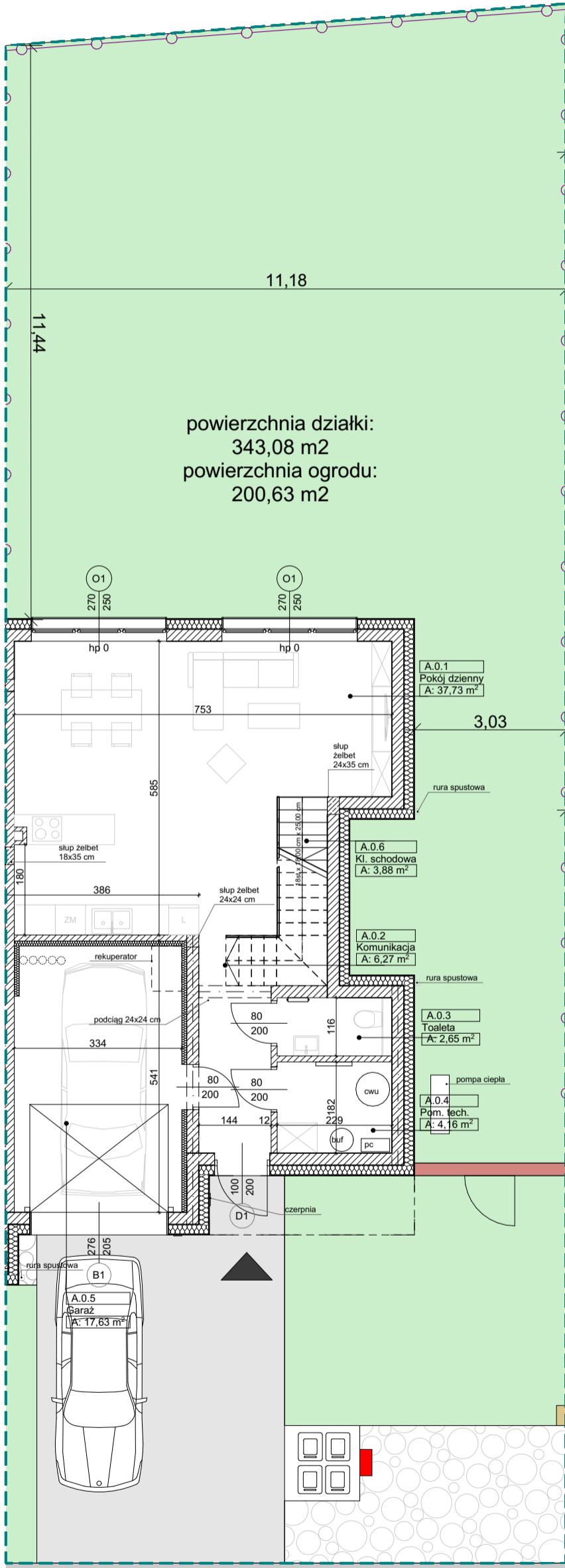
PARTER 1:100
